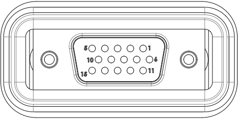
DB15 FEMALE
